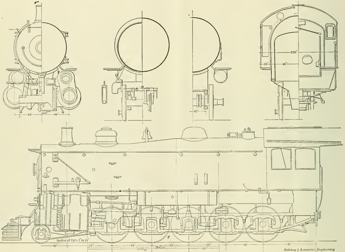
DETAILS OF BALDWIN TANDEM—SEE PAGE 274 OF MAY NUMBER.
